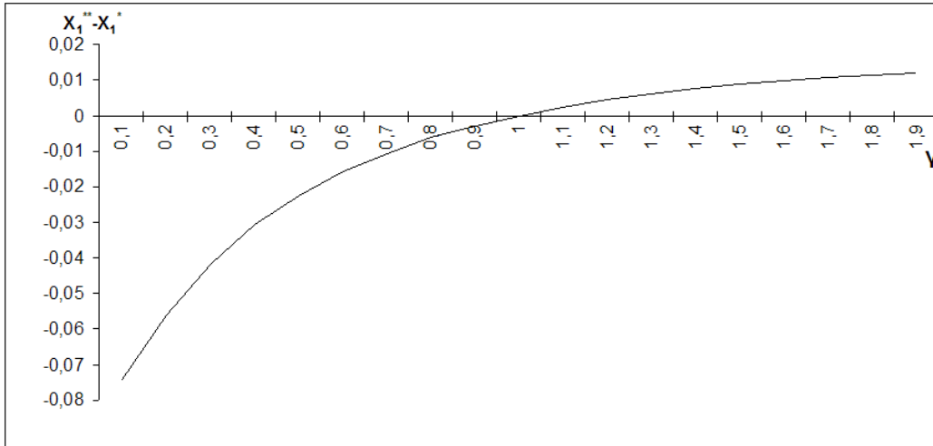
Figure 6: \frac{\psi}{\Delta p} = 1, \bar{p} = 0,9
