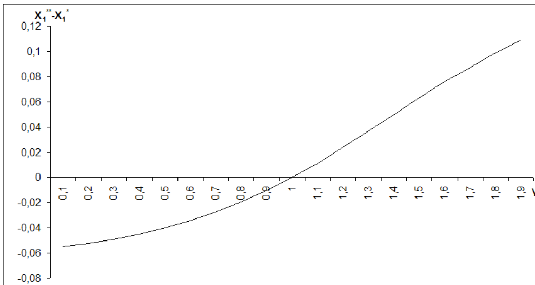
Figure 7: \frac{\psi}{\Delta p} = 1, \bar{p} = 0,2
