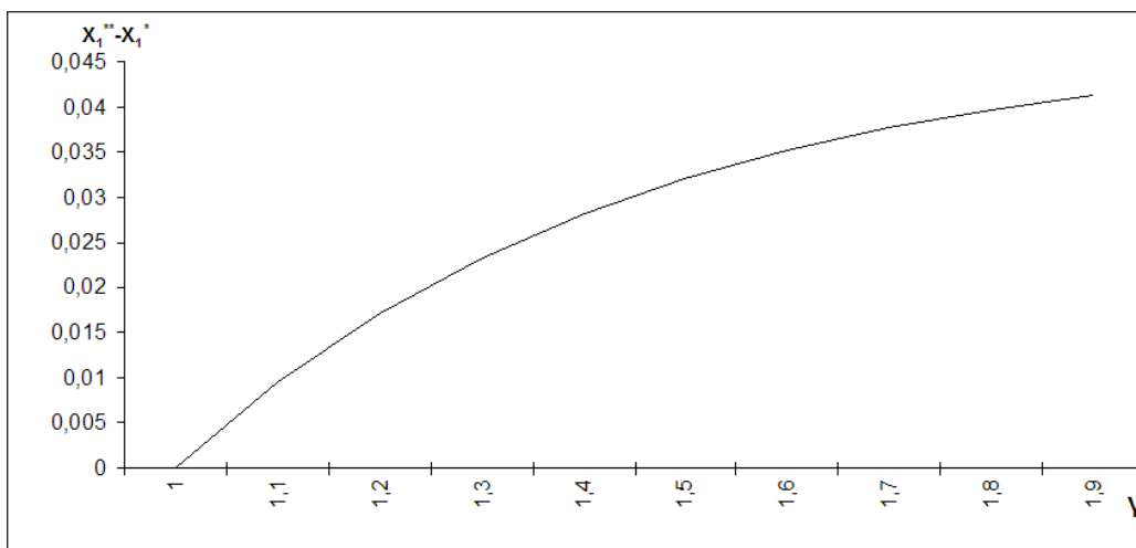
Figure 8: \frac{\psi}{\Delta p} = 10, \bar{p} = 0,9
